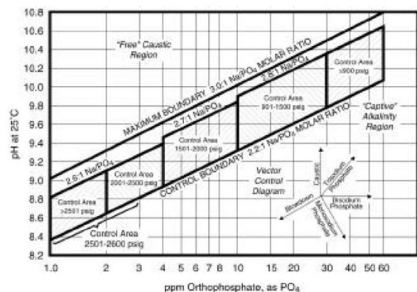
Figure 1: Control diagram for a coordinated phosphate/pH program.
