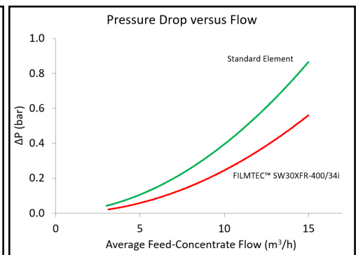
Figure 2: Element differential pressure versus flowrate for SW30XFR-400/34i and Standard Element
