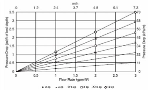
Figure 2: Pressure Drop
