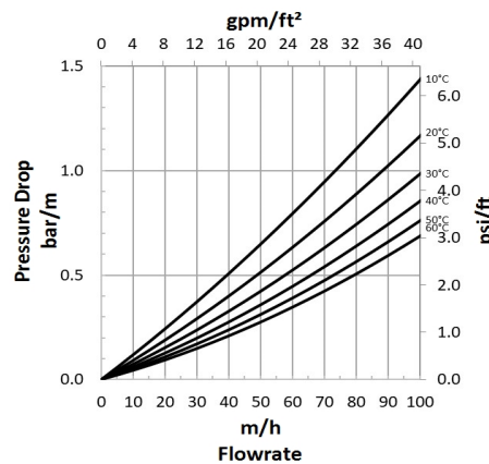
Figure 1: Pressure Drop
