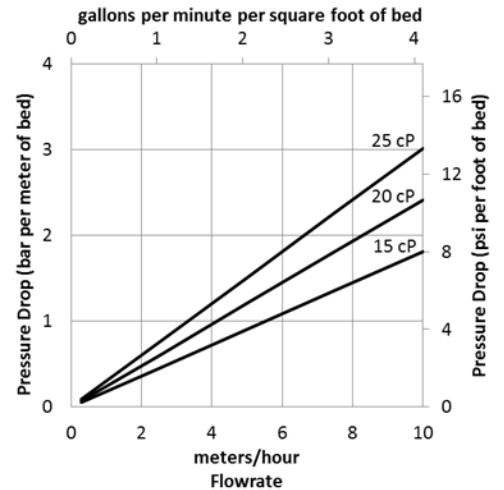
Figure 2: Pressure Drop
