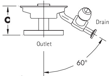
In-line Base with Flange Outlet Connection
