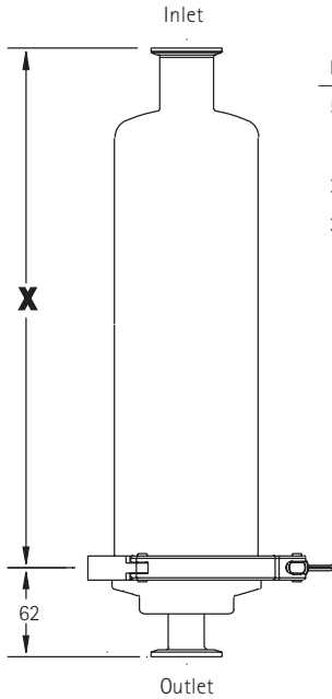
In-line Housing with Ferrule Outlet Connection
