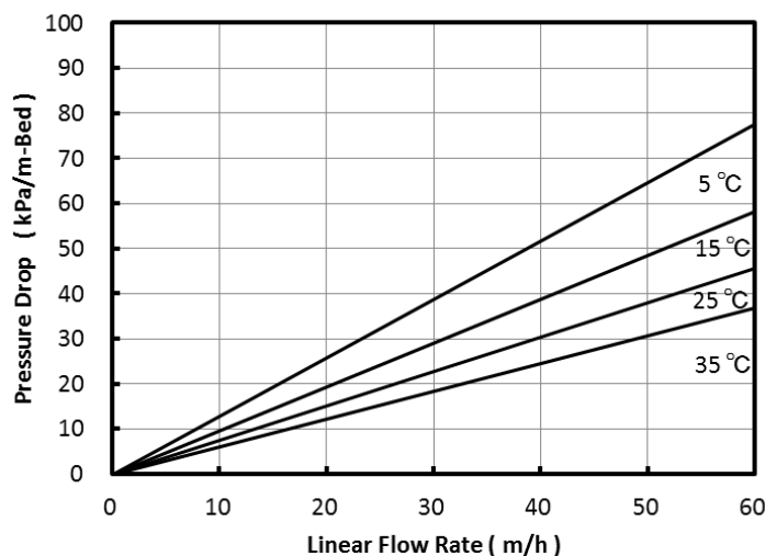
Fig. 1 Pressure Drop of UBK10HUP
