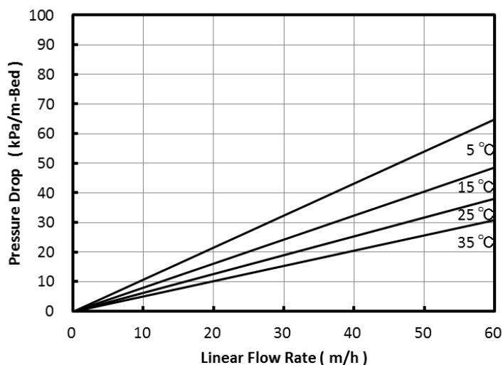
Fig. 1 Pressure Drop of UBA1200H
