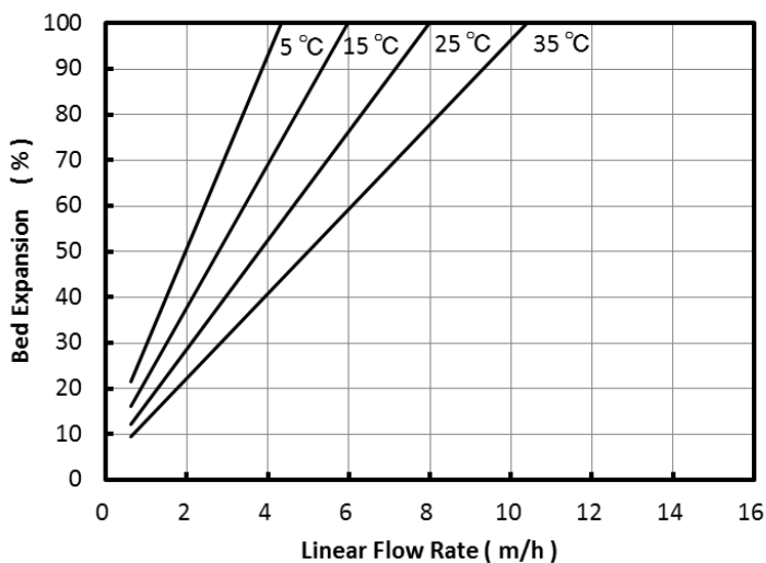
Fig. 2 Bed Expansion of UBA1200H
