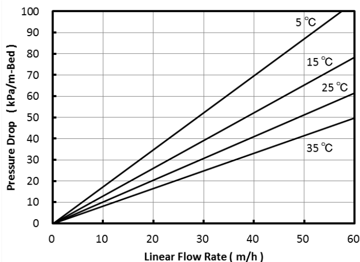
Fig. 1 Pressure Drop of PA308L
