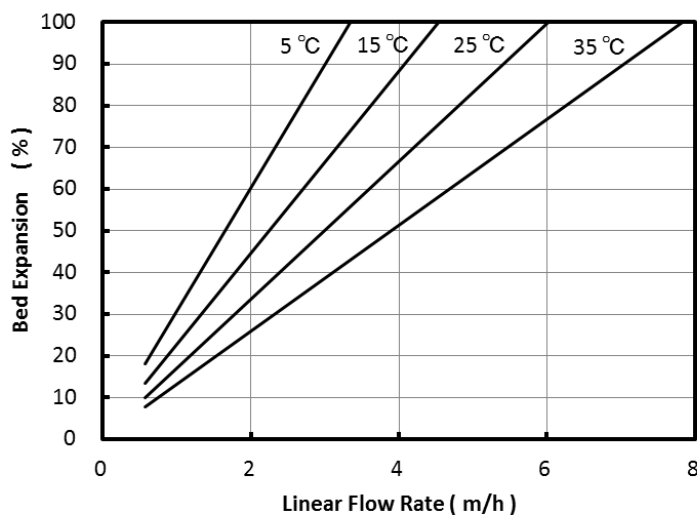
Fig. 2 Bed Expansion of PA308L
