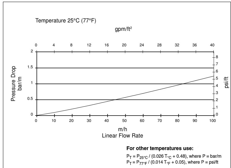
Figure 2. Pressure drop
