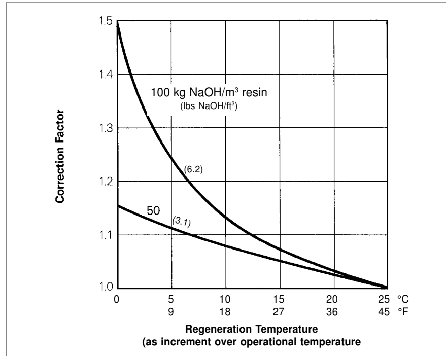
Figure 11. Silica leakage correction for regeneration temperature
