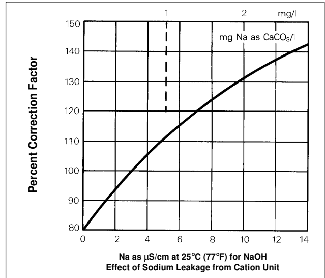
Figure 6. Sodium leakage correction for co-current operation
