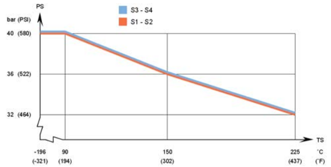
CB30AQ – UL approval pressure/temperature graph
